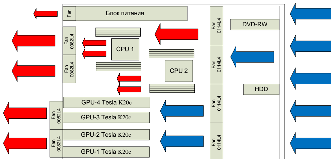
Fig. 2. PHCS system block case cooling scheme
