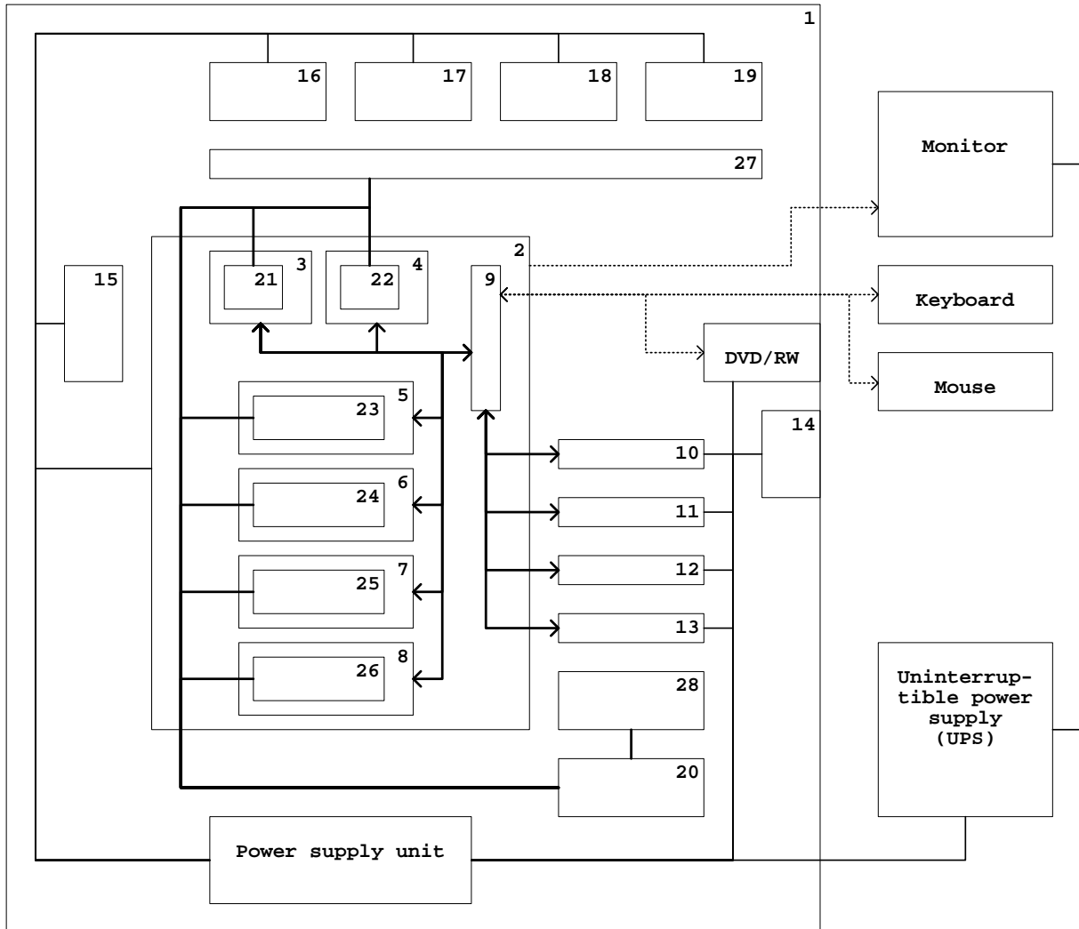
Fig. 3. Structural scheme of a personal hybrid computer system with liquid cooling
