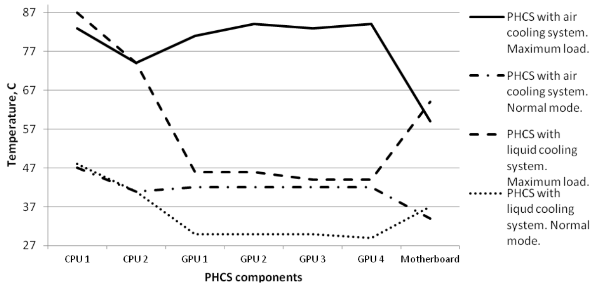
Fig. 6. The results of measurements of personal hybrid computing system heating components
