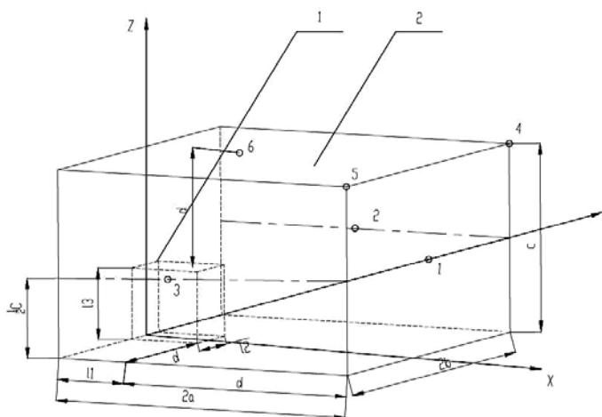
1- reference parallelepiped, 2 - measuring surface
