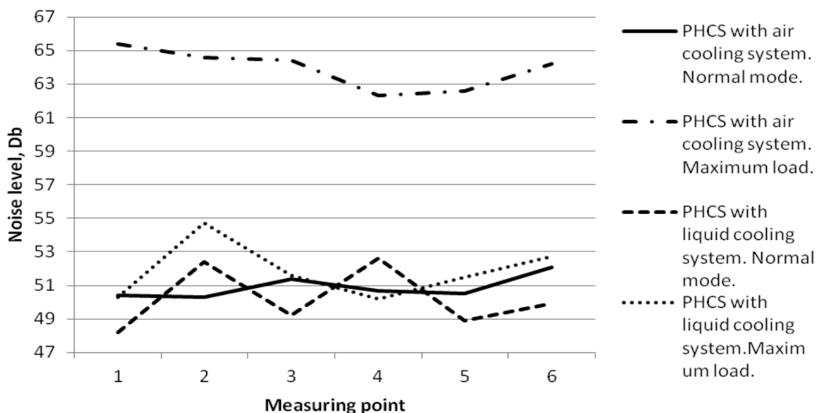
Fig. 5. The results of measurements of sound power of personal hybrid computing system
